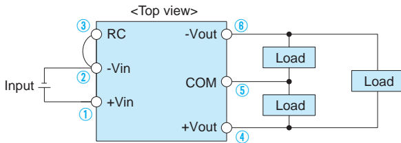
Fig.1.1 Pin Configuration (MG15)
