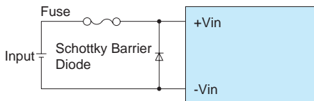
Fig.3.2 Connecting a Reverse Voltage Protection Circuit
