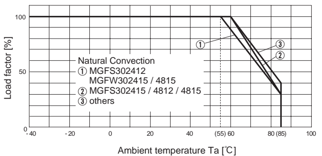
Fig.8.5 Derating Curve for Convection Cooling (Rated Input Voltage)
