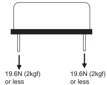
Fig.6.1 Stress onto Pins
